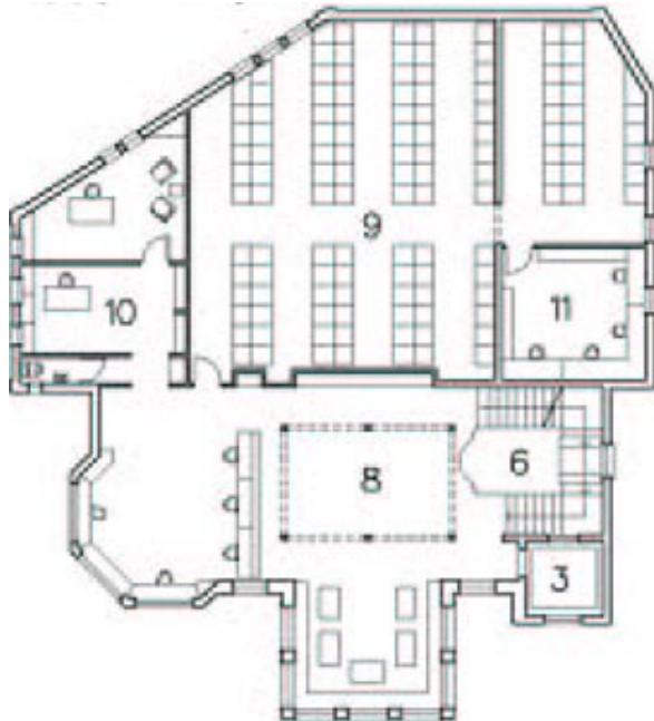
first floor plan - music lending library 8 catalogues and librarian counter 9 notes, scores, books 10 administration 11 librarian's room
